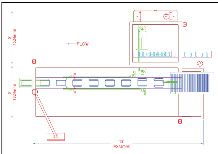
Standard Range Floorplan
